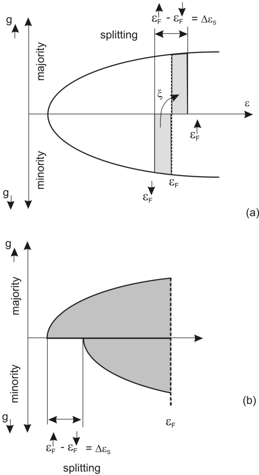
Fig. 1. Density of states in the rigid band model: (a) assuming two different Fermi levels for the two subbands; (b) assuming the same Fermi energy, which is actually the real physical case. The two situations are mathematically equivalent, but the formalism developed based on model (a) is easiest for computations.
