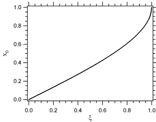
Fig. 8. Solutions (62) of equation (61).
