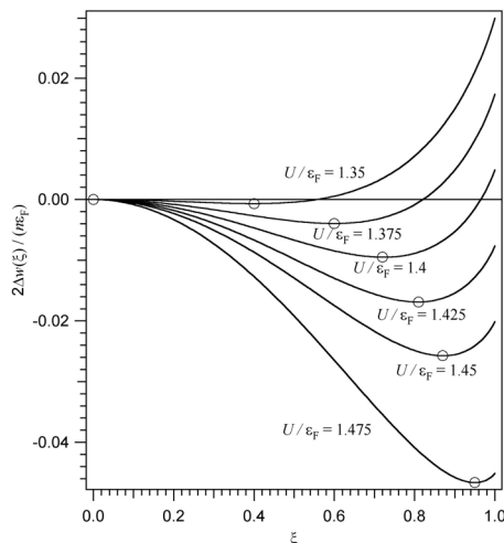
Fig. 4. Energy dependence on the asymmetry parameter, for the 3D case.
