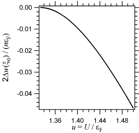
Fig. 6. Energy gain of the ferromagnetic state, as function on the ratio between the Hubbard term U and the Fermi energy \varepsilon_F .
