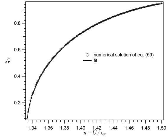
Fig. 5. Variation of the equilibrium asymmetry parameter \xi_0 as function on the ratio between the Hubbard term U and the Fermi energy \varepsilon_F .
