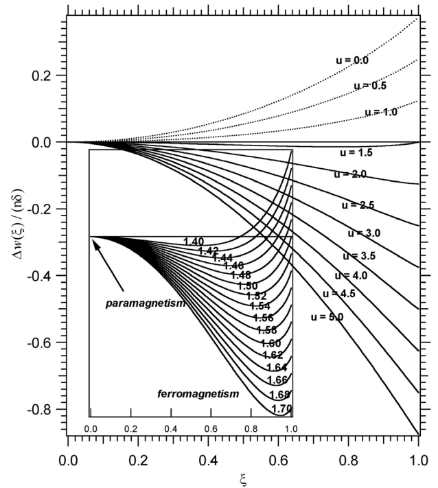
Fig. 9. Energy difference between the ferromagnetic and the paramagnetic state, as function on the asymmetry \xi , for several values of the parameter u = U/\delta (ratio between Hubbard energy and DOS half-width). The dotted curves on the large graph represent cases where the Stoner criterion is not satisfied. The insert represents energy curves in the region of u yielding ferromagnetism with incomplete polarization.
