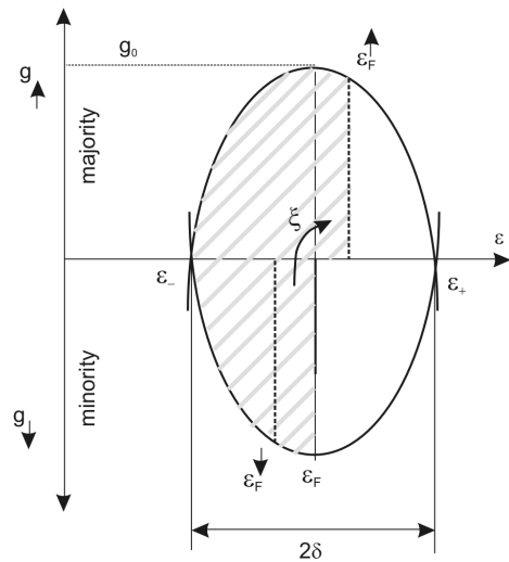
Fig. 7. The parabolic density of states, half-filled for zero polarization.
