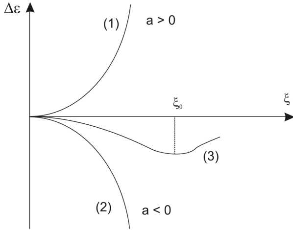
Fig. 2. Energy variation as function on the asymmetry parameter \xi . Case (1): stable paramagnetic state; case (2): unstable paramagnetic state; case (3) situation where the minimum energy is obtained for a given value of asymmetry \xi_0 .
