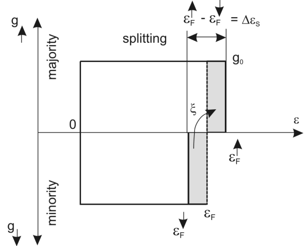
Fig. 3. Spin-resolved density of states for the ideal 2D case.
