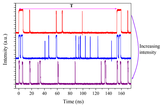
Fig. 11. Evolution of the laser output intensity for increasing pumping powers.
