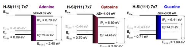
Fig. 4. Energy level alignment at the interface between adenine (left), cytosine (middle), and guanine (right) layers and the Si(111)7x7 substrates.
