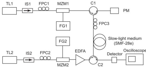
Fig.5 Experiment of low distortion Brillouin slow light in optical fibers using AM modulation
