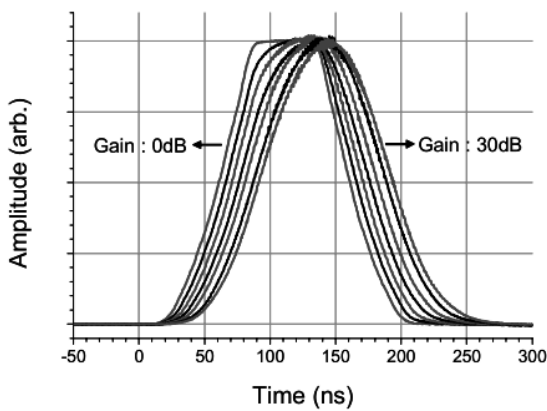
Fig.3 Traces of the probe pulses of different Brillouin gains for standard fiber
