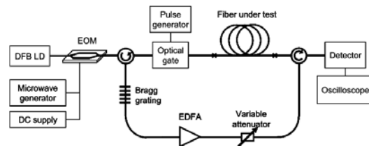
Fig.2. Configuration to measure variable pulse delay from SBS in an optical fiber
