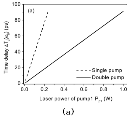
Fig.11 The result of experiment (a) the relationship between time delay and the power of pump1 (b) the relationship between pulse broadening and the power of pump1
