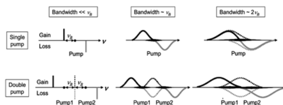
Fig.8 Comparison of gain and loss spectra in single and double Brillouin pumps
